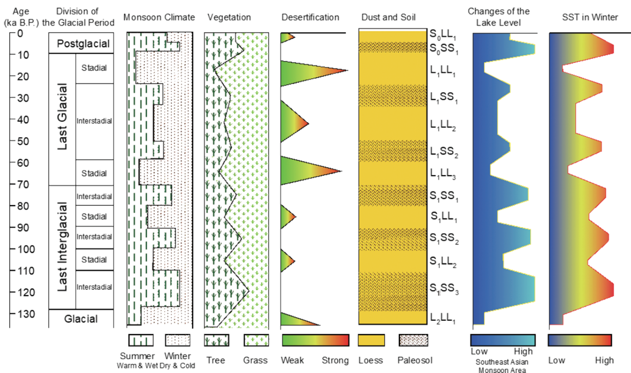
Fig. 5. Environmental changes in East Asia controlled by the monsoon climate changes.
