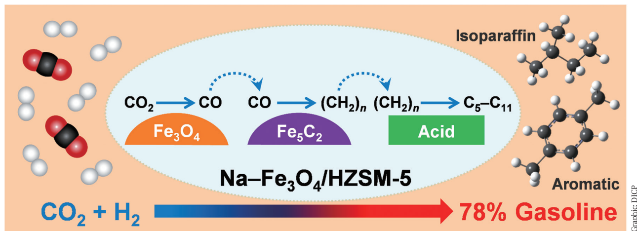
Schematic diagram of CO 2 hydrogenation catalytic reaction.
