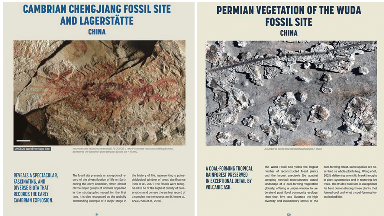
Figure 3. The first pages of the Cambrian Chengjiang Fossil Site and Lagerstätten, and the Permian Vegetation of the Wuda Fossil Site respectively as a brief introduction in the publication of the first and second 100 IUGS Geological Heritage Sites.
